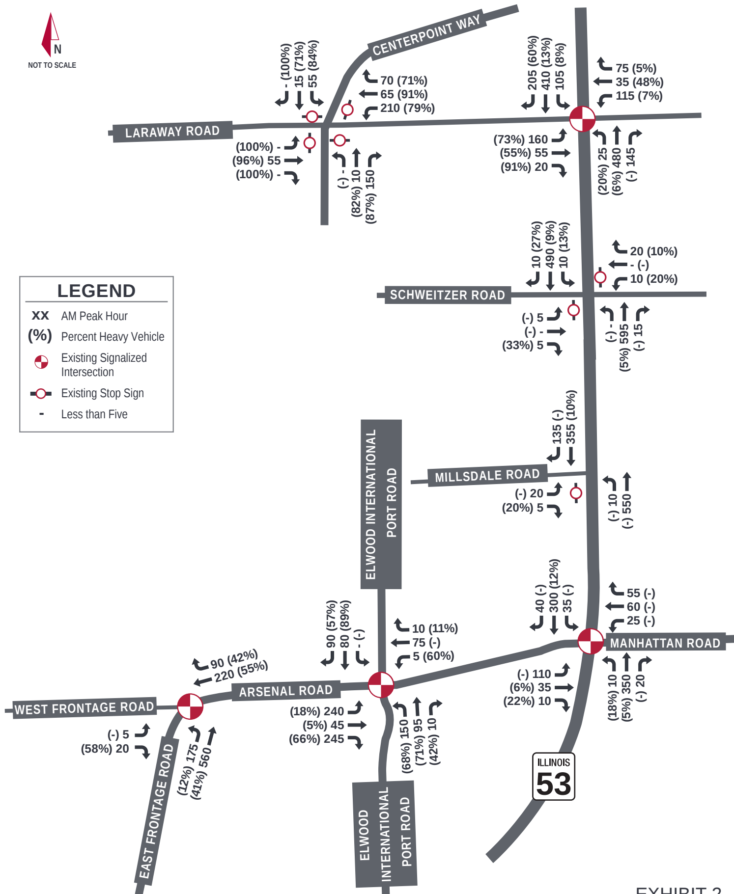
EXHIBIT 2 EXISTING 2015 TRAFFIC VOLUMES MORNING PEAK HOUR
